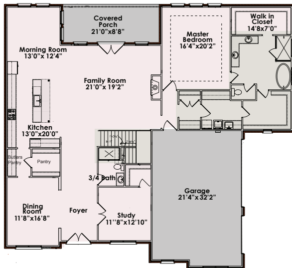
Main Level Floor 2,779sf
