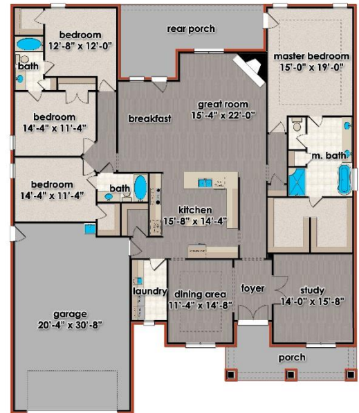
Main Level Floor
