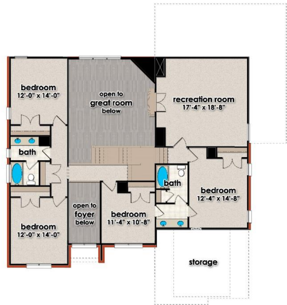
Upper Level Floor
